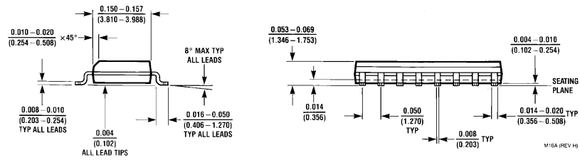
Plastic Surface-Mount Package (M) Order Number LP365M NS Package Number M16A
