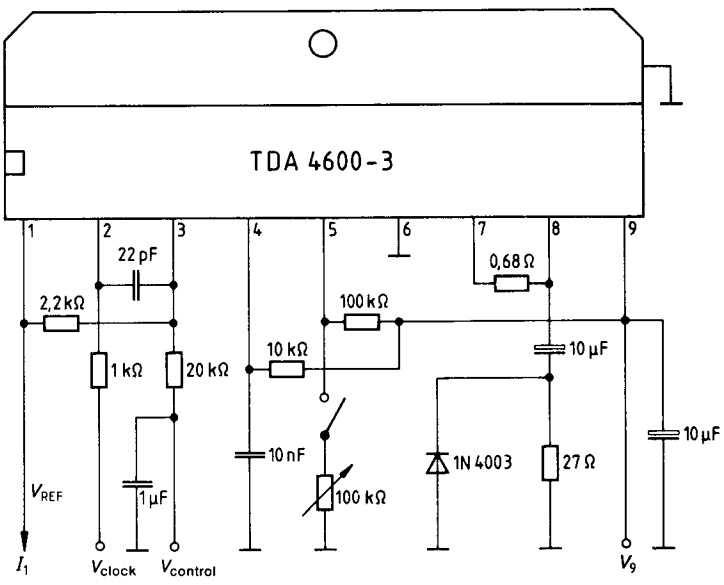
Measurement circuit 1
